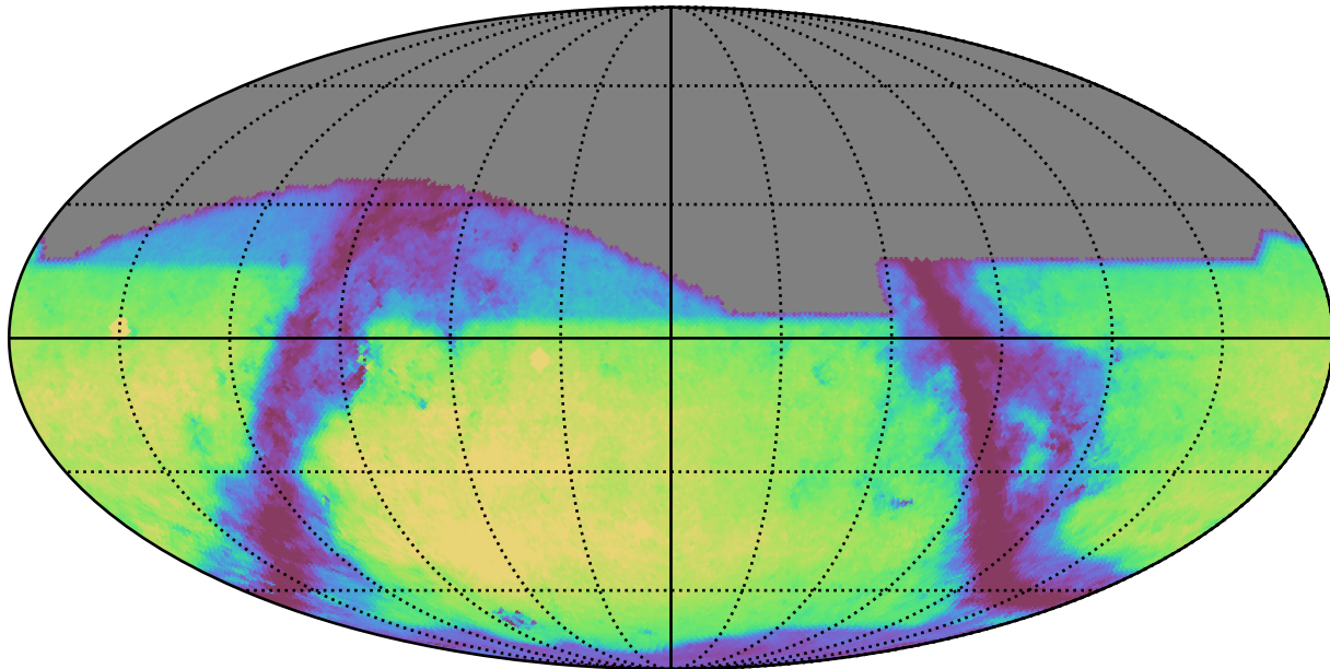
too_100_4v3.4_10yrs r: GalaxyCountsMetricExtended
