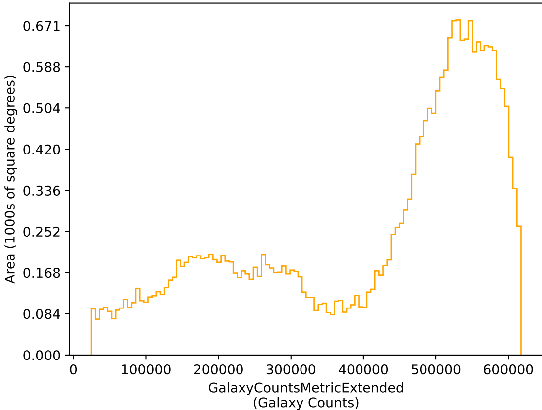
too_100_4v3.4_10yrs r: GalaxyCountsMetricExtended
