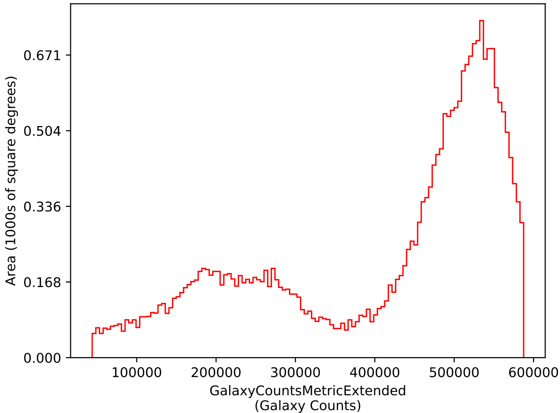
too_100_4v3.4_10yrs i: GalaxyCountsMetricExtended
