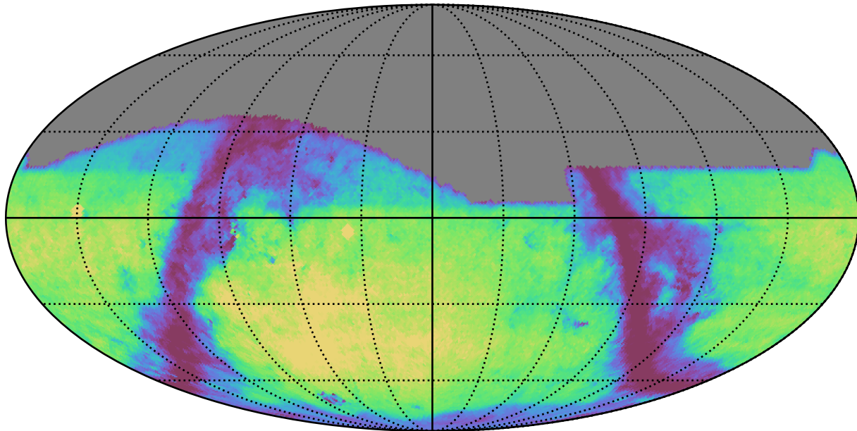
too_100_4v3.4_10yrs g: GalaxyCountsMetricExtended
