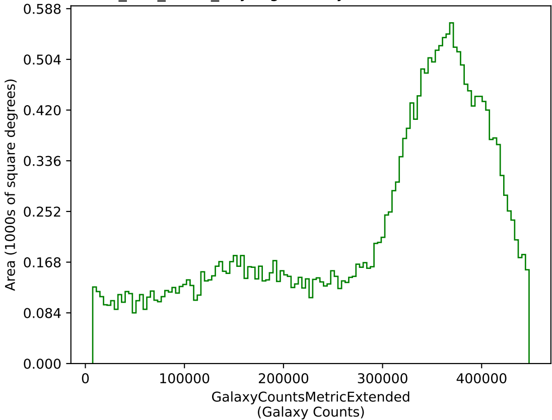
too_100_4v3.4_10yrs g: GalaxyCountsMetricExtended
