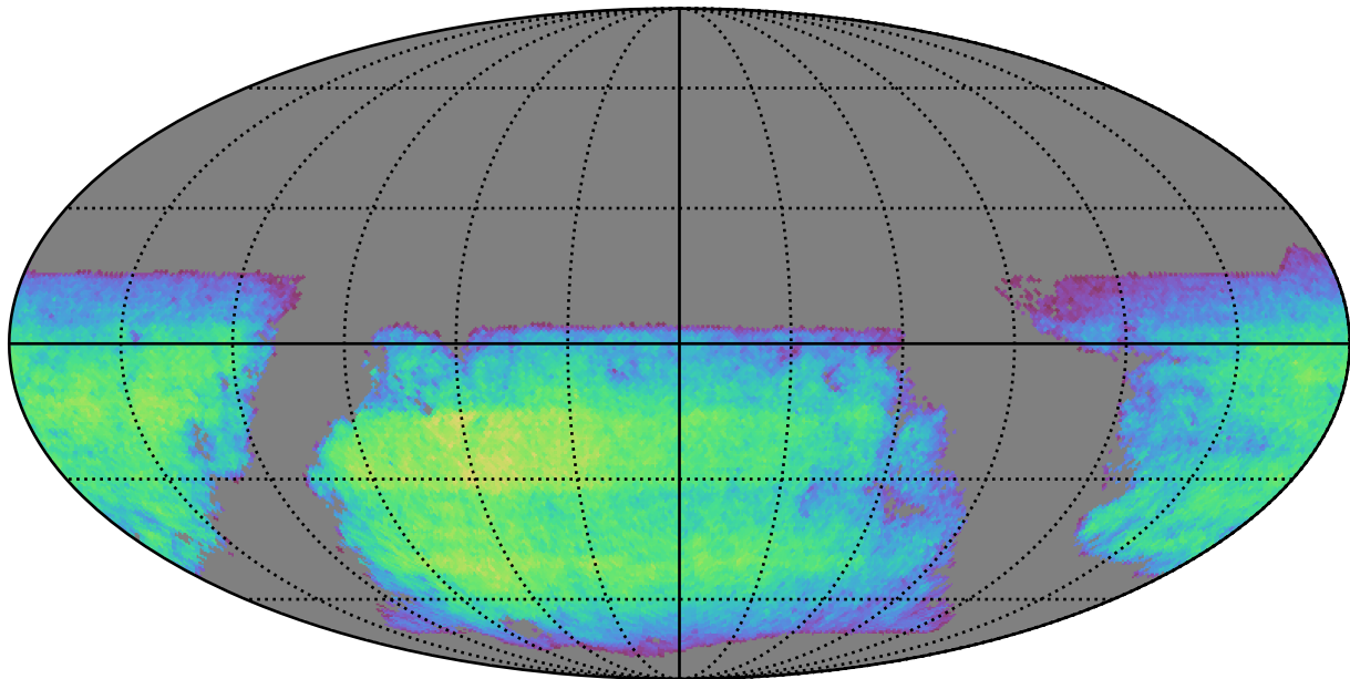
too_100_4v3.4_10yrs i band non-DD year 9: ExgalM5WithCuts
