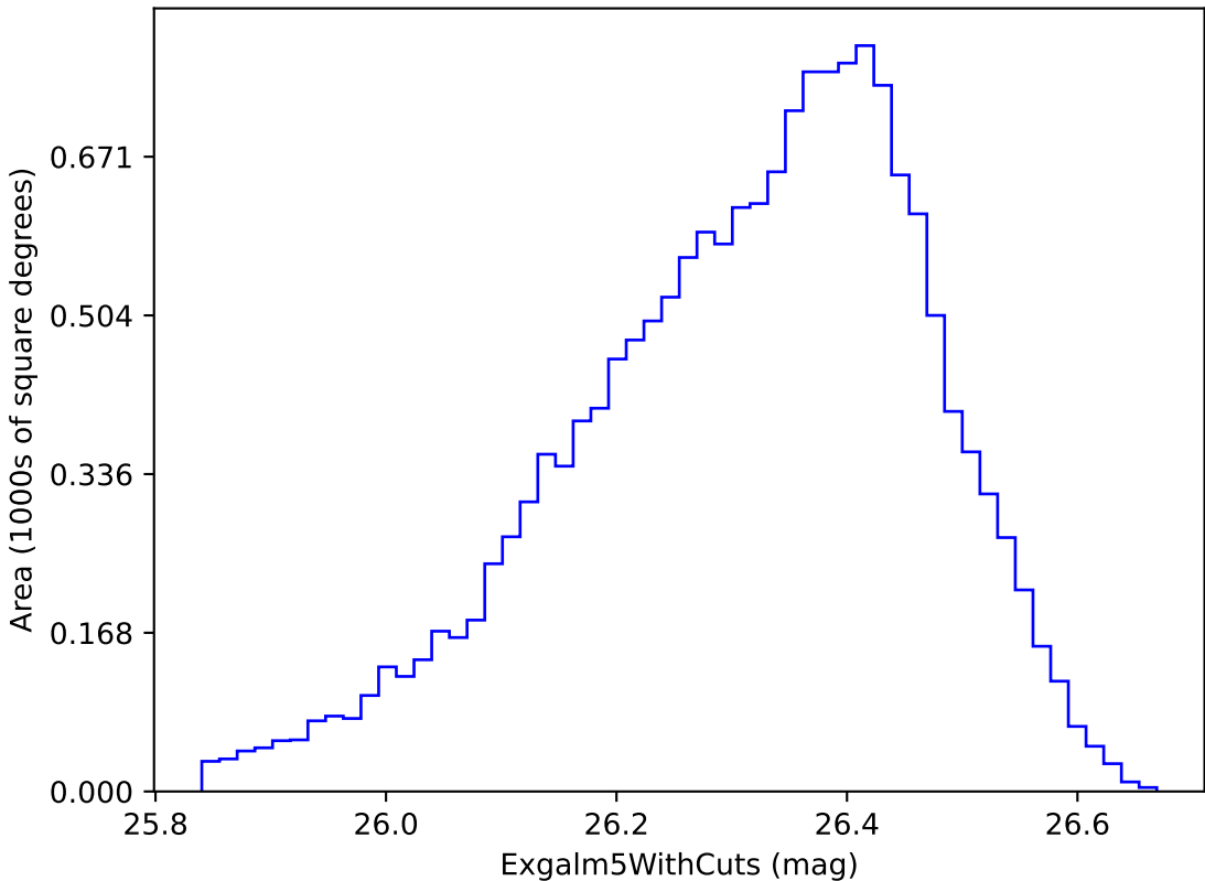
too_100_4v3.4_10yrs i band non-DD year 9: ExgalM5WithCuts
