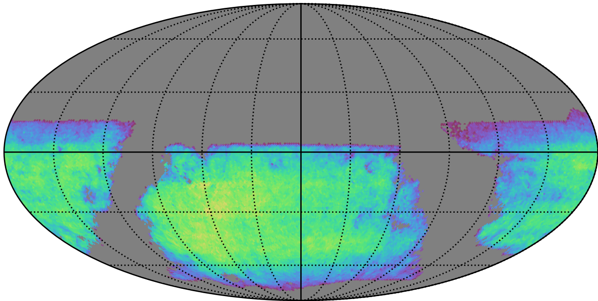
too_100_4v3.4_10yrs i band non-DD year 8: ExgalM5WithCuts
