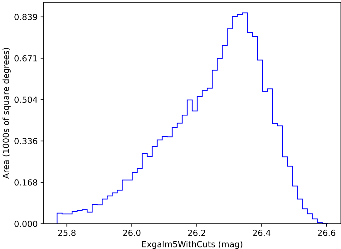
too_100_4v3.4_10yrs i band non-DD year 8: ExgalM5WithCuts
