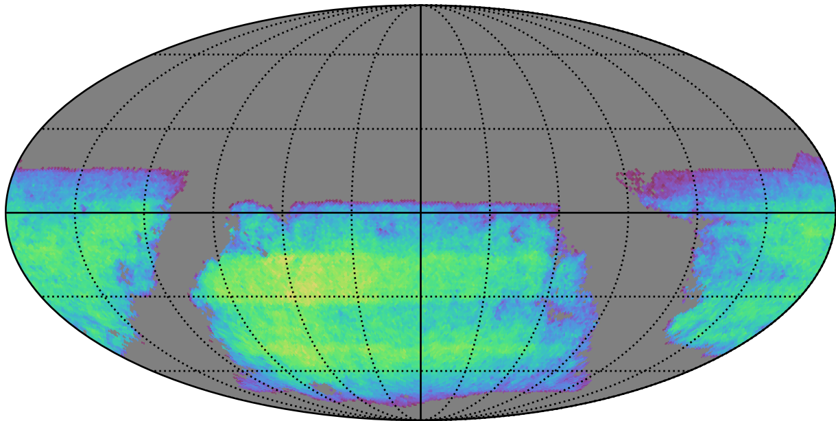
too_100_4v3.4_10yrs i band non-DD year 7: ExgalM5WithCuts
