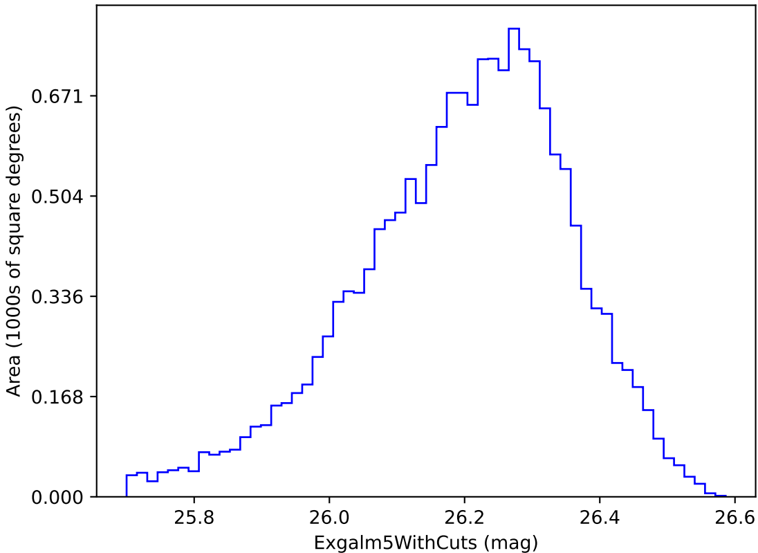
too_100_4v3.4_10yrs i band non-DD year 7: ExgalM5WithCuts
