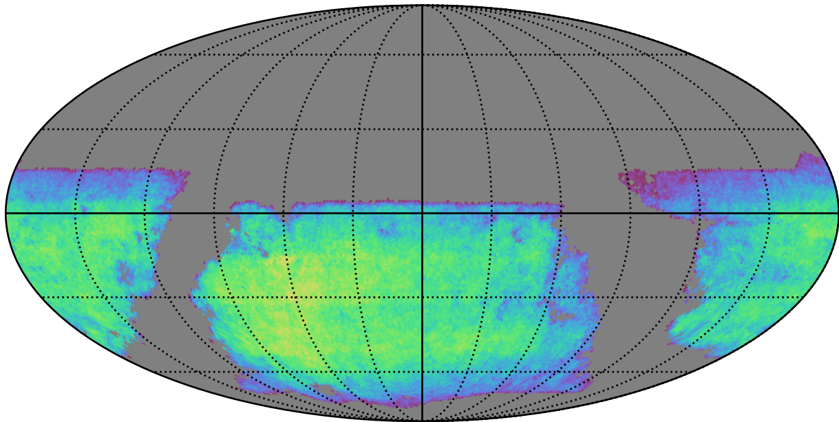
too_100_4v3.4_10yrs i band non-DD year 6: ExgalM5WithCuts
