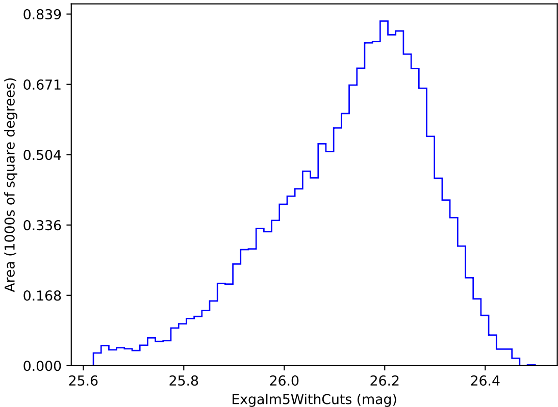
too_100_4v3.4_10yrs i band non-DD year 6: ExgalM5WithCuts
