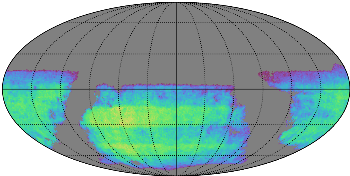
too_100_4v3.4_10yrs i band non-DD year 5: ExgalM5WithCuts
