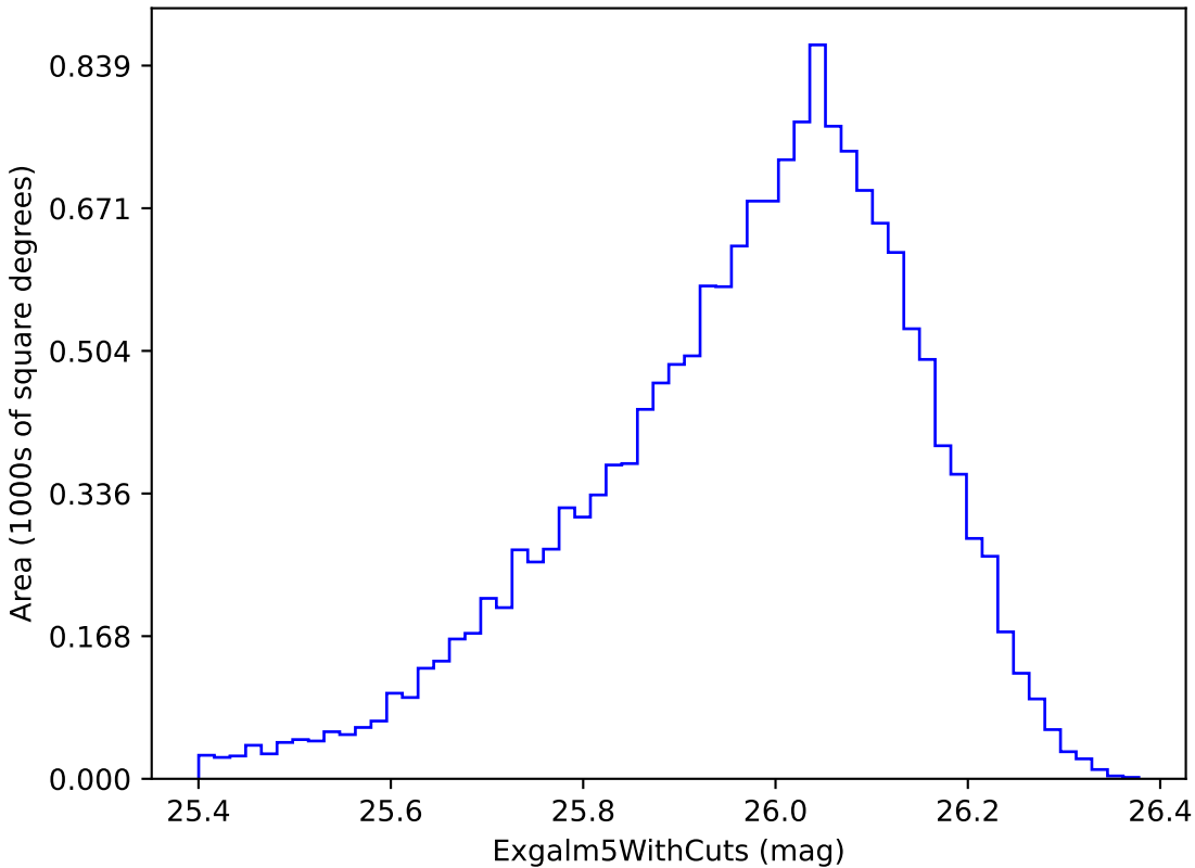
too_100_4v3.4_10yrs i band non-DD year 4: ExgalM5WithCuts
