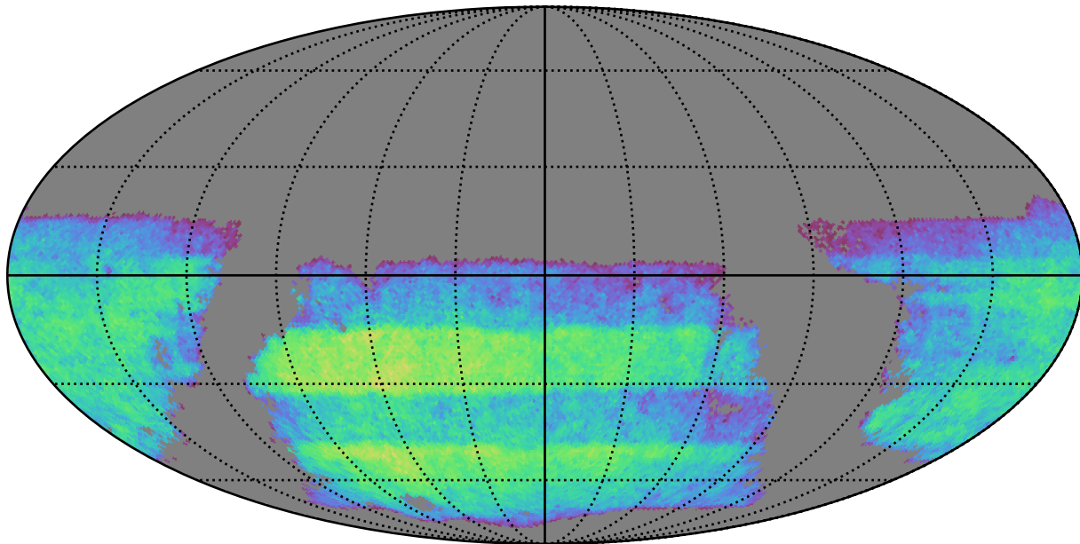
too_100_4v3.4_10yrs i band non-DD year 3: ExgalM5WithCuts
