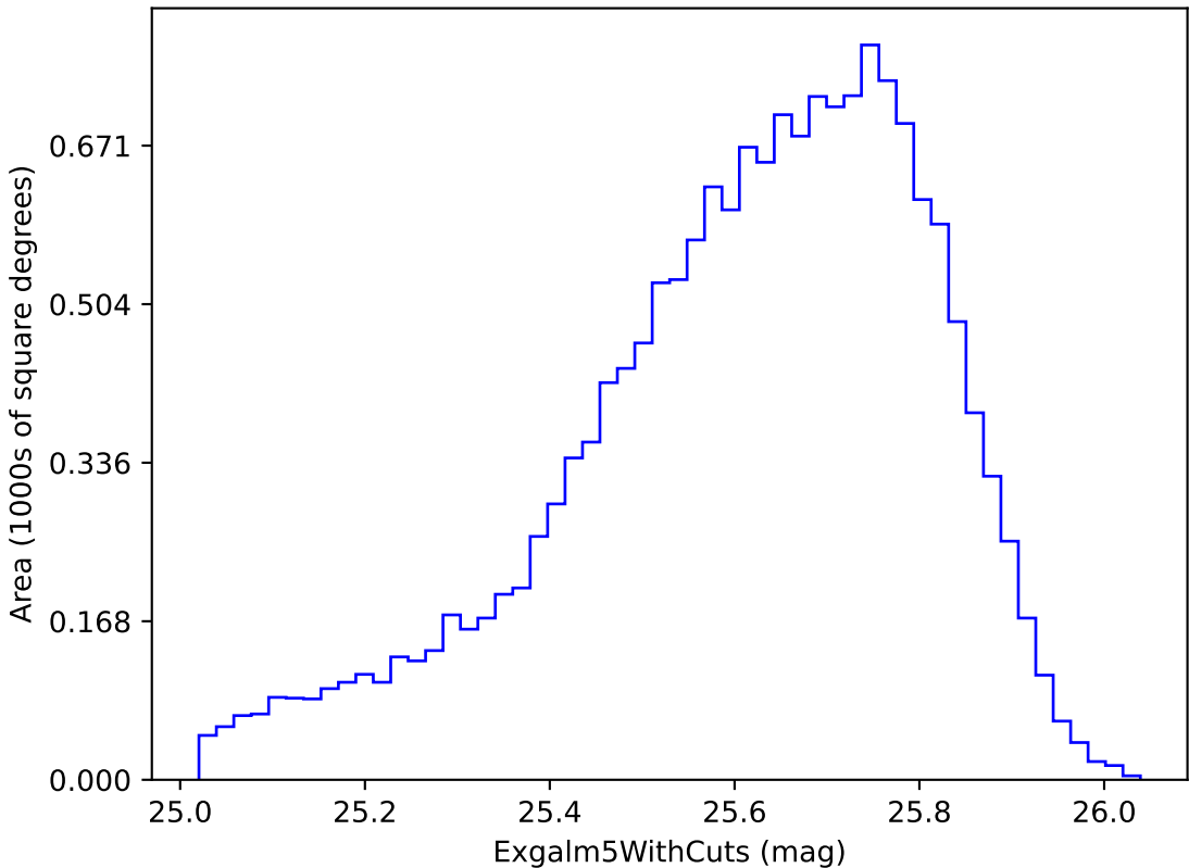
too_100_4v3.4_10yrs i band non-DD year 2: ExgalM5WithCuts
