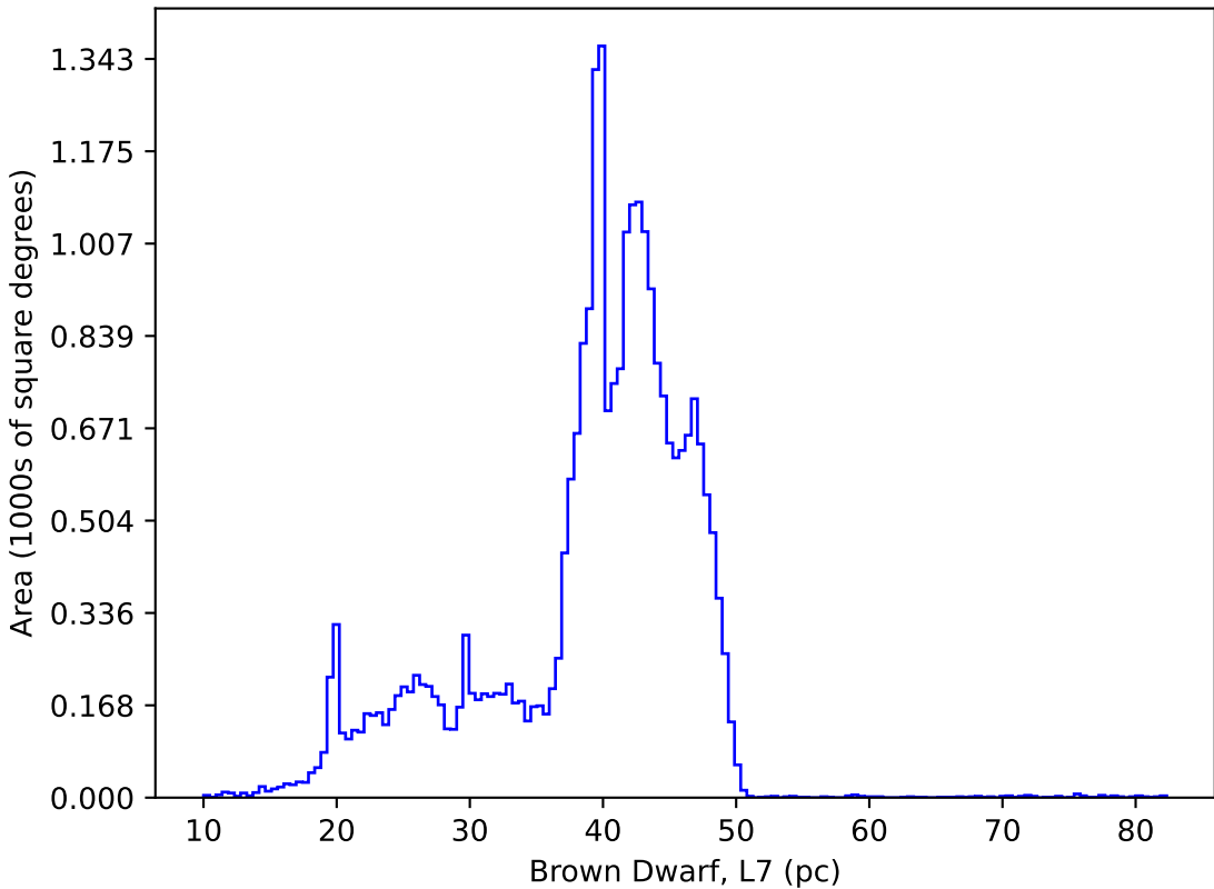
too_100_4v3.4_10yrs : Brown Dwarf, L7
