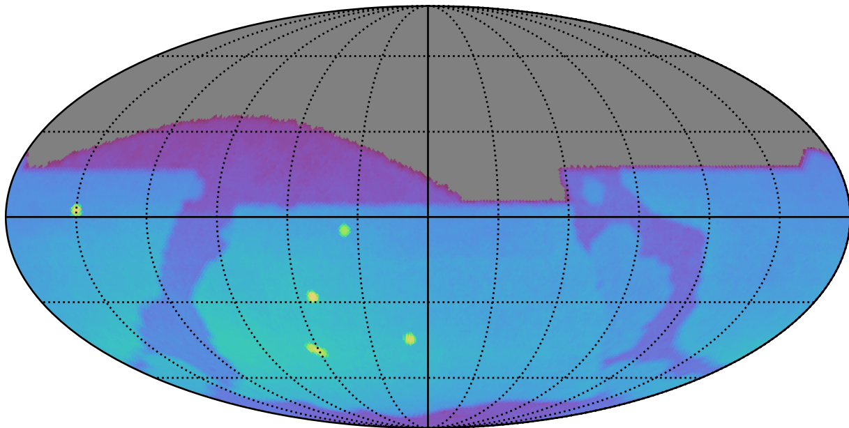
too_100_4v3.4_10yrs : Brown Dwarf, L4
