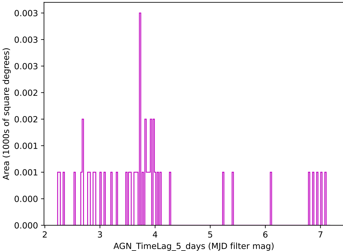
too_100_4v3.4_10yrs z band: AGN_TimeLag_5_days
