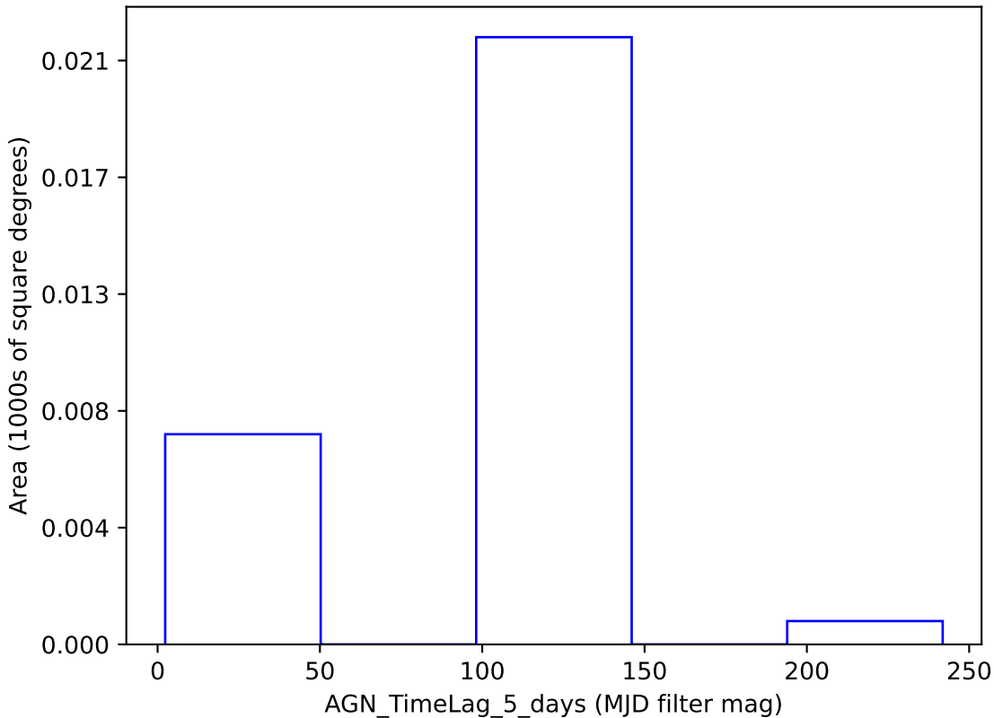
too_100_4v3.4_10yrs y band: AGN_TimeLag_5_days
