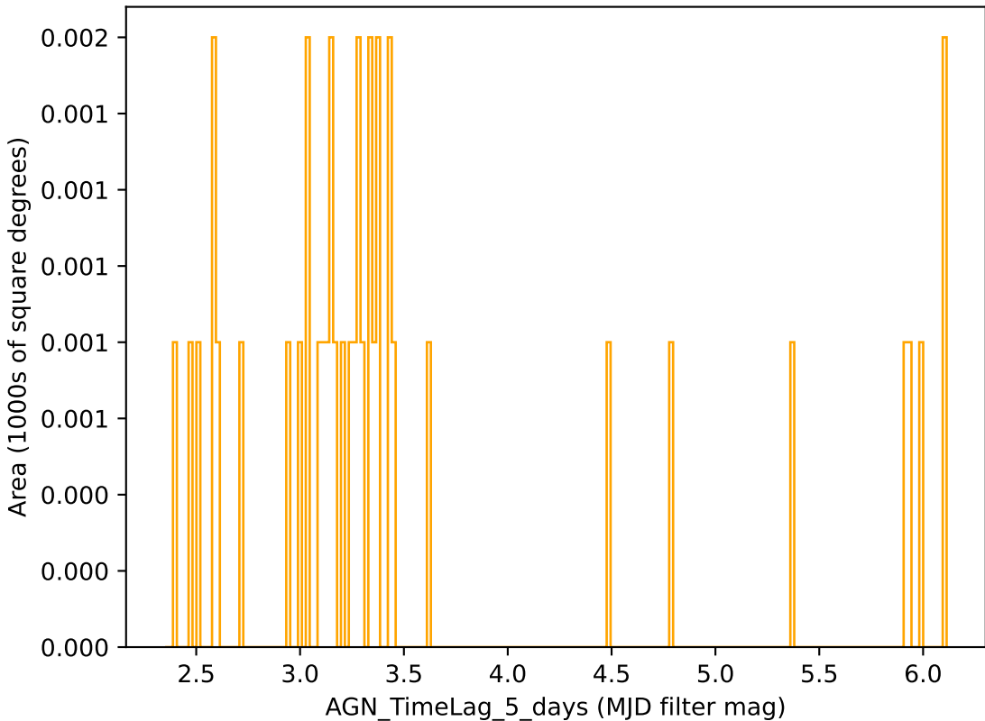
too_100_4v3.4_10yrs r band: AGN_TimeLag_5_days
