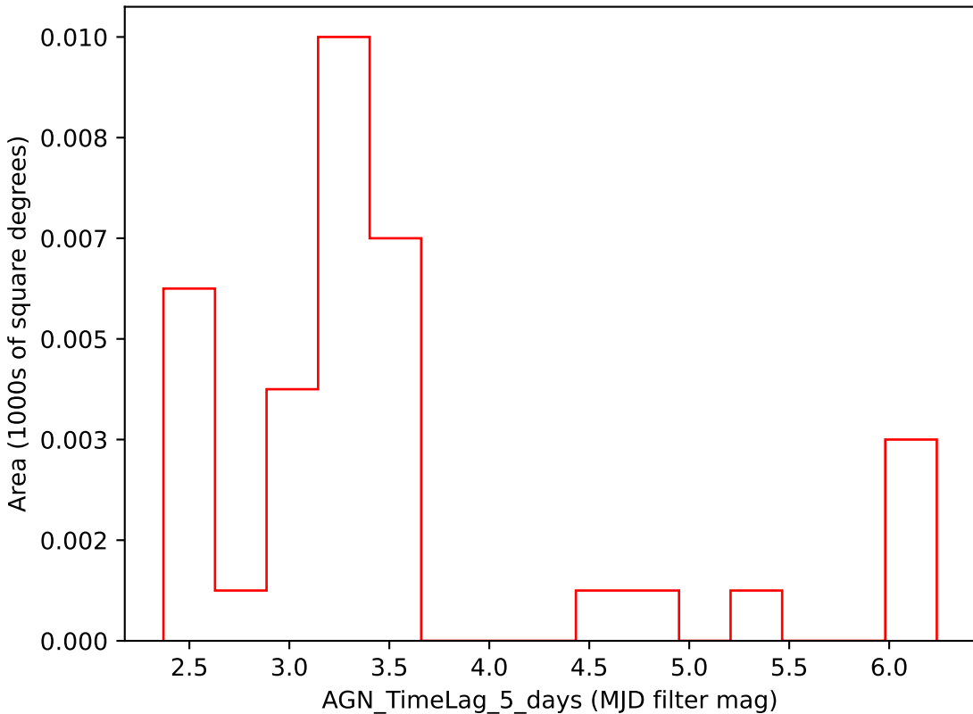
too_100_4v3.4_10yrs i band: AGN_TimeLag_5_days
