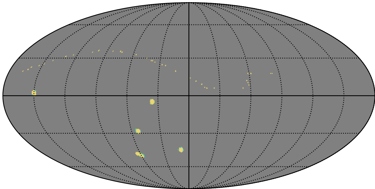
too_100_4v3.4_10yrs all bands: AGN_TimeLag_5_days
