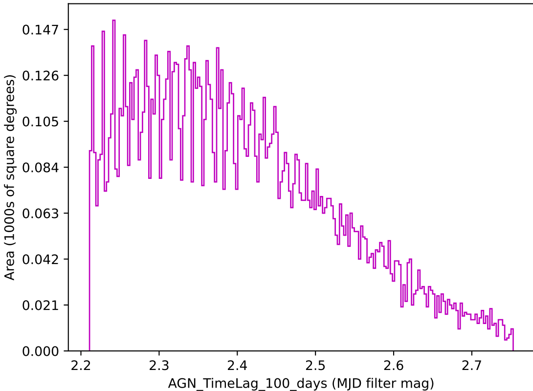
too_100_4v3.4_10yrs z band: AGN_TimeLag_100_days
