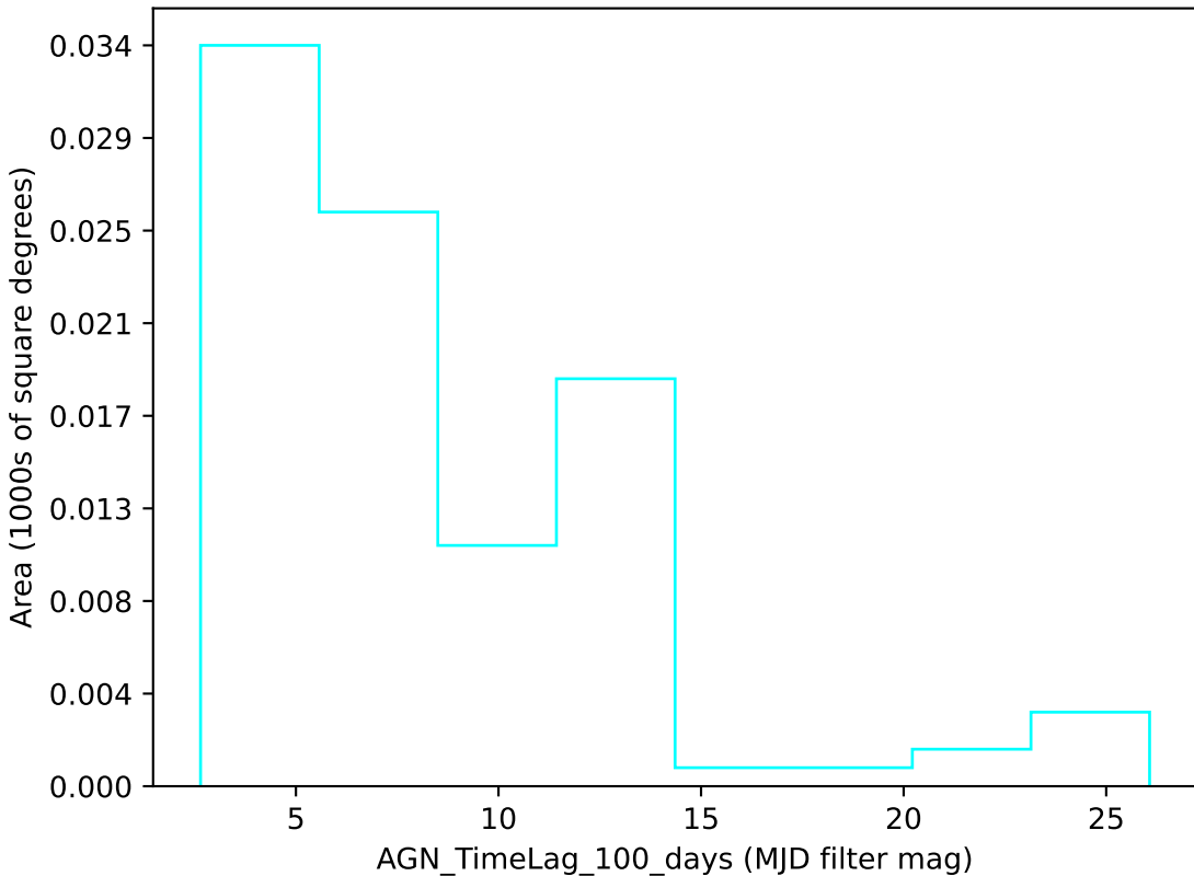
too_100_4v3.4_10yrs u band: AGN_TimeLag_100_days
