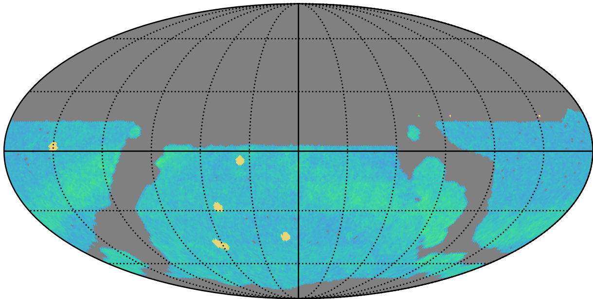
too_100_4v3.4_10yrs r band: AGN_TimeLag_100_days
