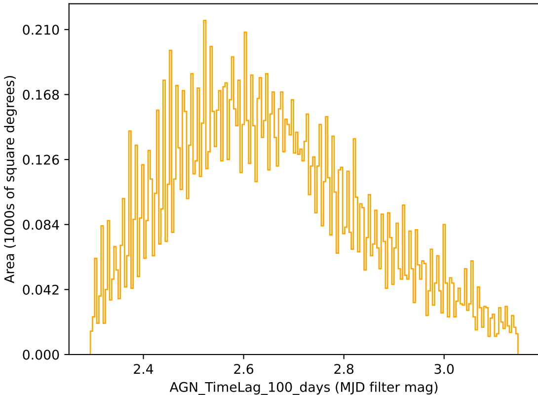
too_100_4v3.4_10yrs r band: AGN_TimeLag_100_days
