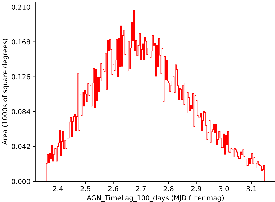
too_100_4v3.4_10yrs i band: AGN_TimeLag_100_days
