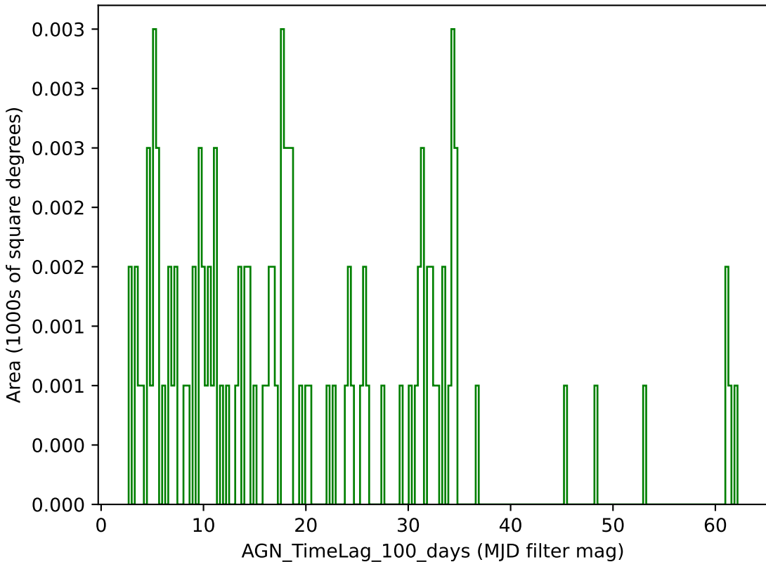
too_100_4v3.4_10yrs g band: AGN_TimeLag_100_days
