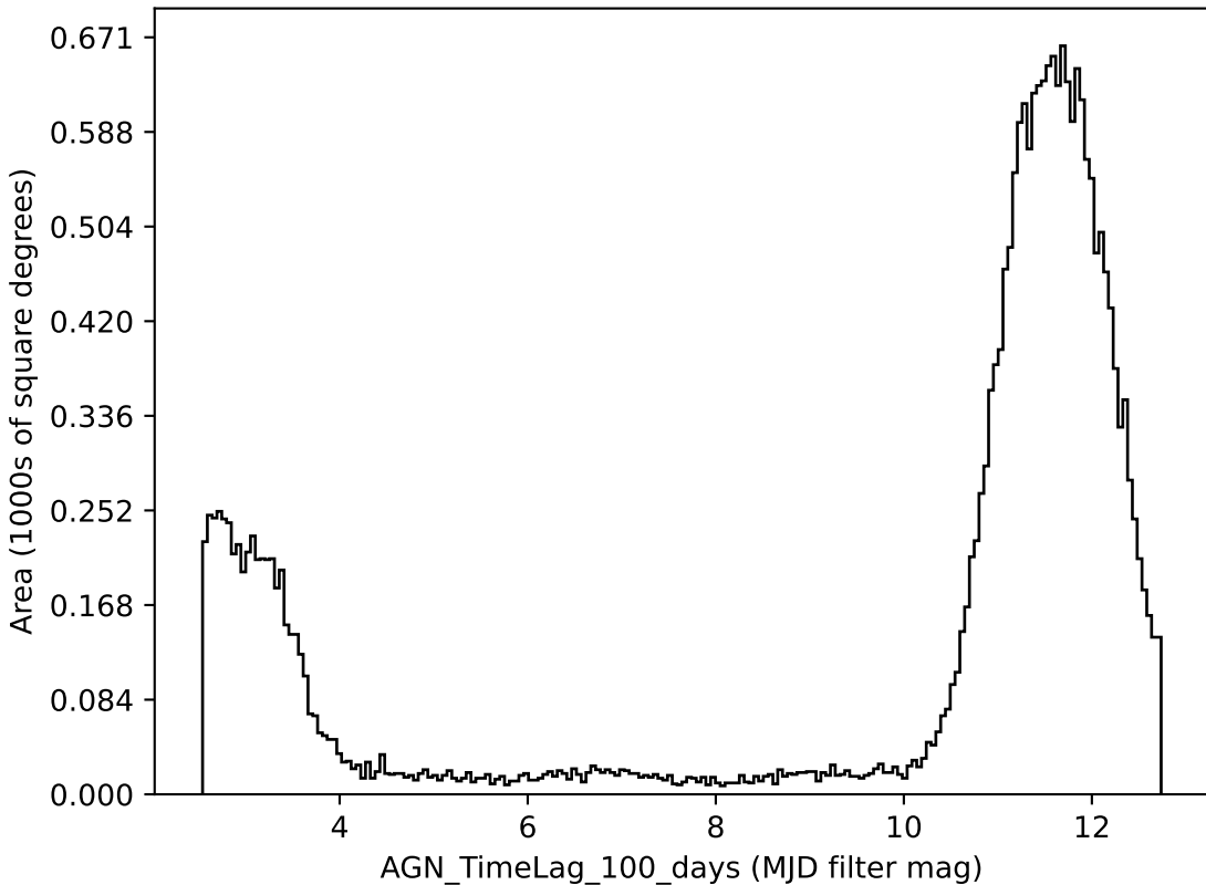
too_100_4v3.4_10yrs all bands: AGN_TimeLag_100_days
