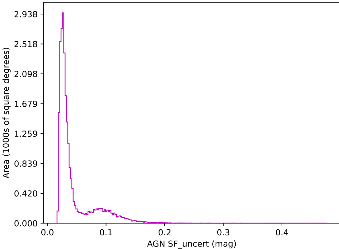
too_100_4v3.4_10yrs z band: AGN SF_uncert
