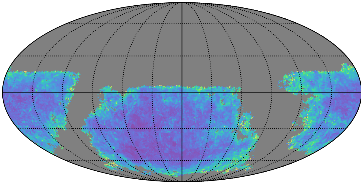
too_100_4v3.4_10yrs u band: AGN SF_uncert
