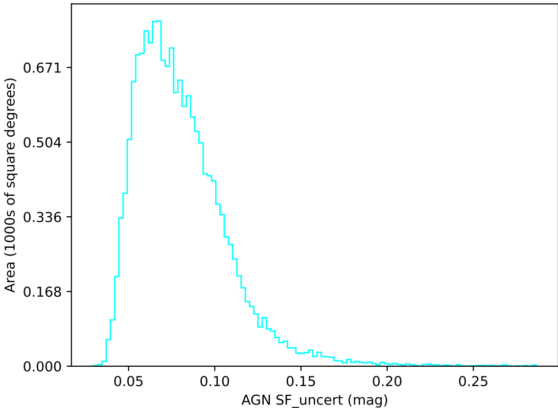
too_100_4v3.4_10yrs u band: AGN SF_uncert
