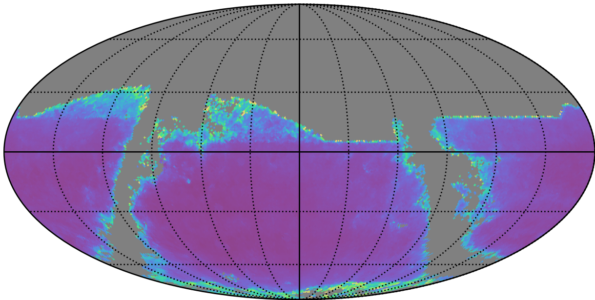
too_100_4v3.4_10yrs r band: AGN SF_uncert
