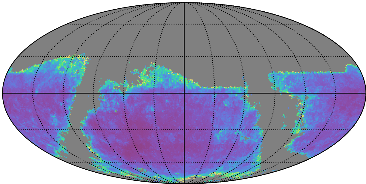
too_100_4v3.4_10yrs g band: AGN SF_uncert
