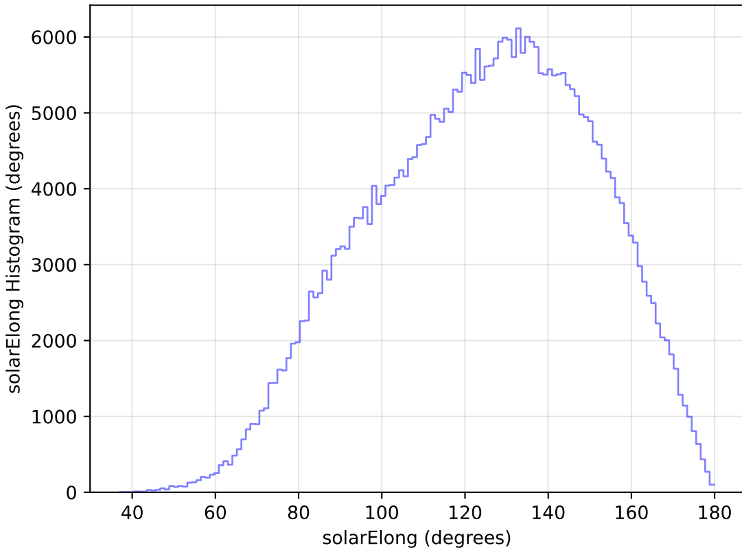
too_100_4v3.4_10yrs WFD y band: solarElong Histogram
