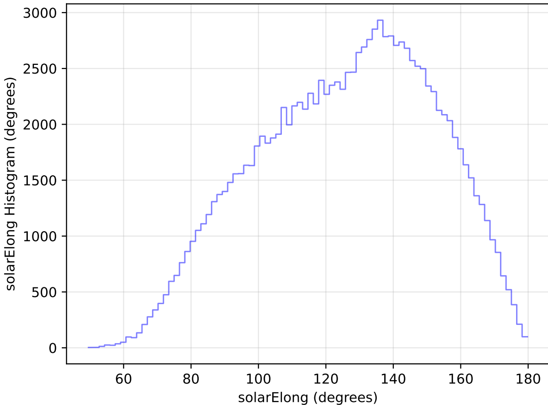
too_100_4v3.4_10yrs WFD u band: solarElong Histogram
