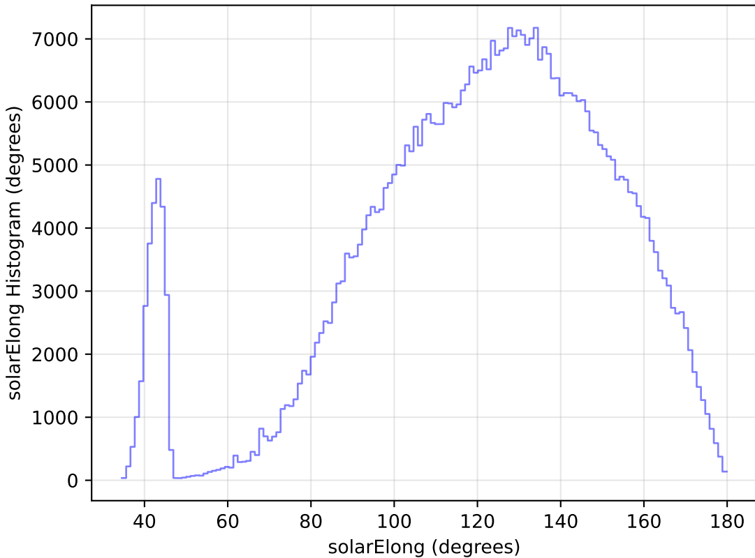
too_100_4v3.4_10yrs WFD i band: solarElong Histogram
