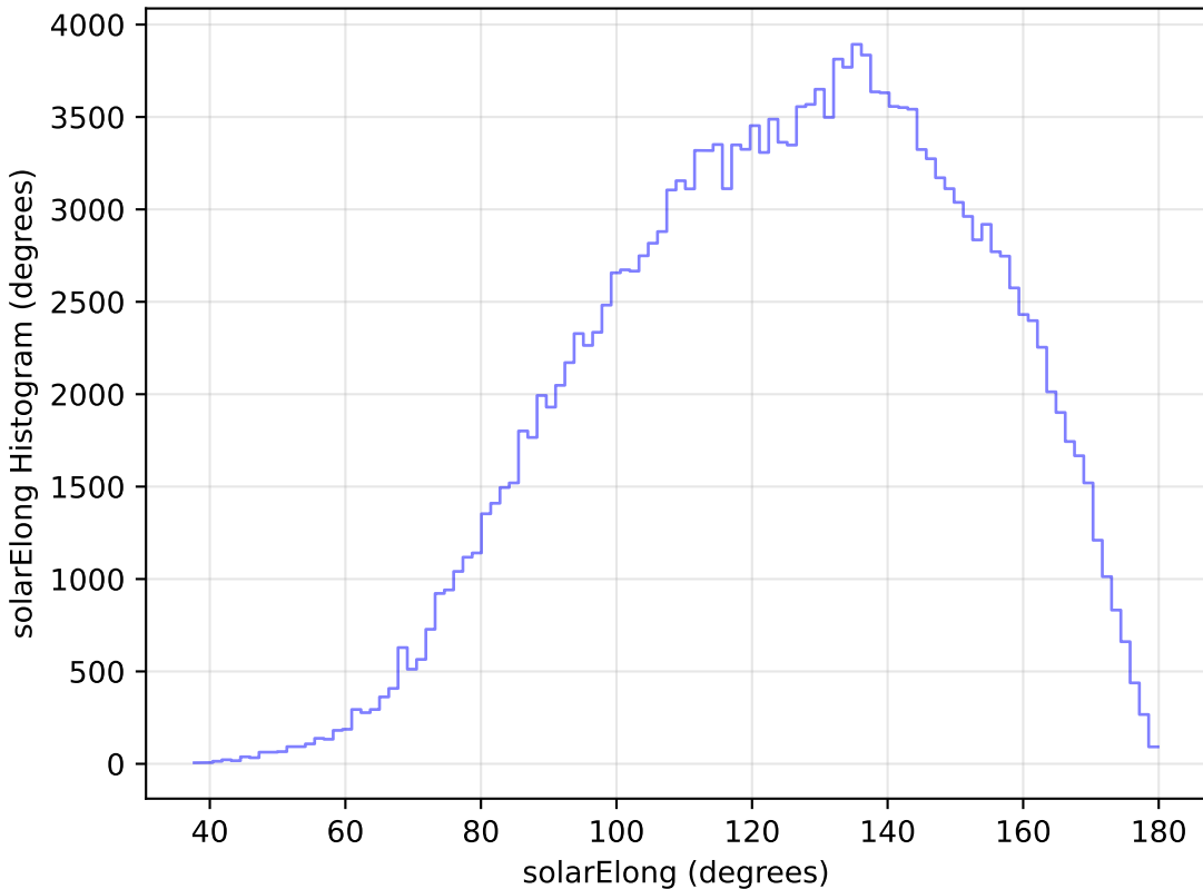
too_100_4v3.4_10yrs WFD g band: solarElong Histogram
