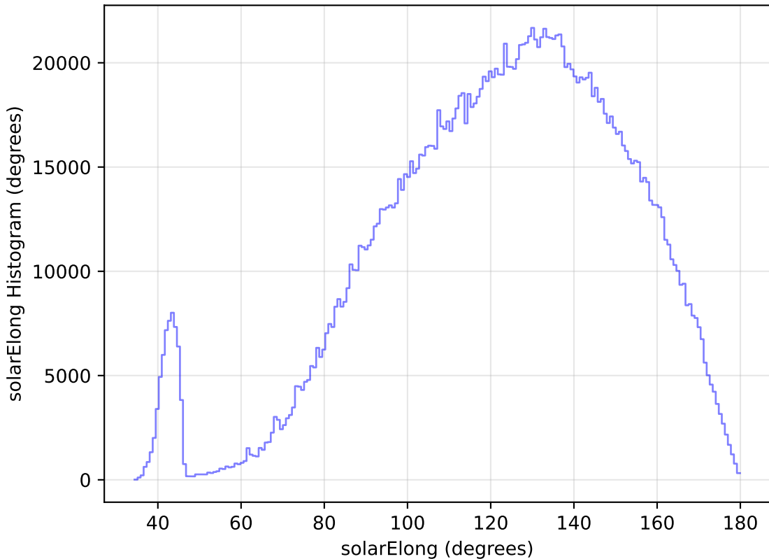
too_100_4v3.4_10yrs WFD all bands: solarElong Histogram
