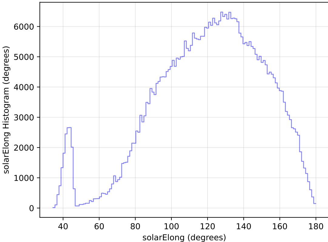
too_100_4v3.4_10yrs All sky z band: solarElong Histogram
