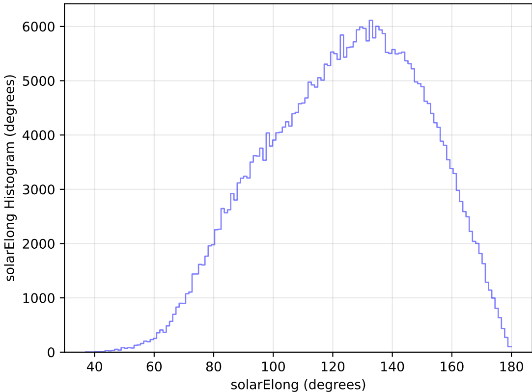
too_100_4v3.4_10yrs All sky y band: solarElong Histogram
