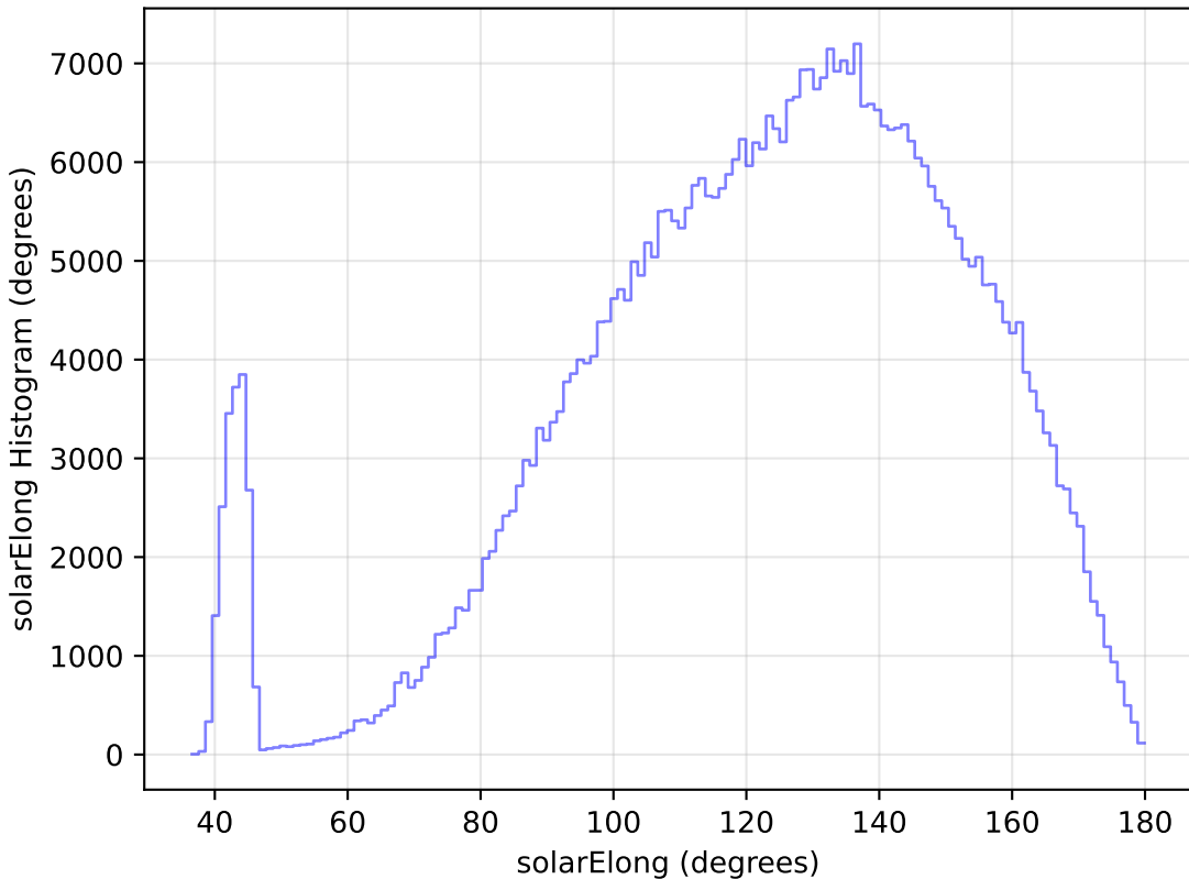
too_100_4v3.4_10yrs All sky r band: solarElong Histogram
