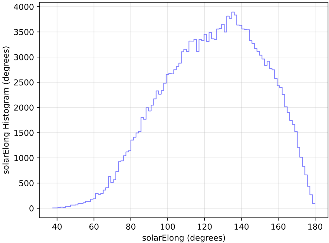
too_100_4v3.4_10yrs All sky g band: solarElong Histogram
