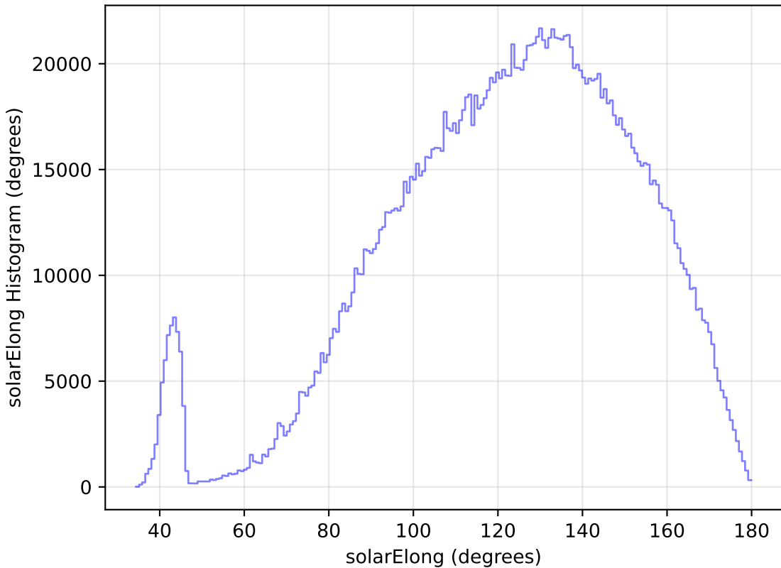
too_100_4v3.4_10yrs All sky all bands: solarElong Histogram
