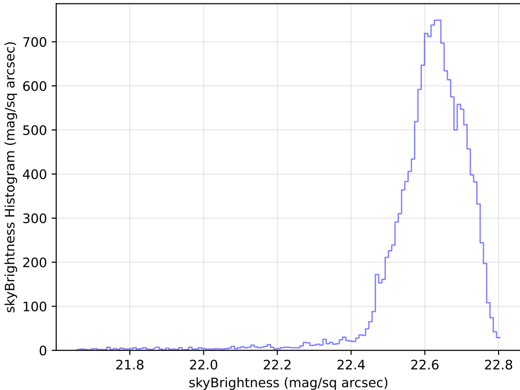
too_100_4v3.4_10yrs Yr 1 u band: skyBrightness Histogram
