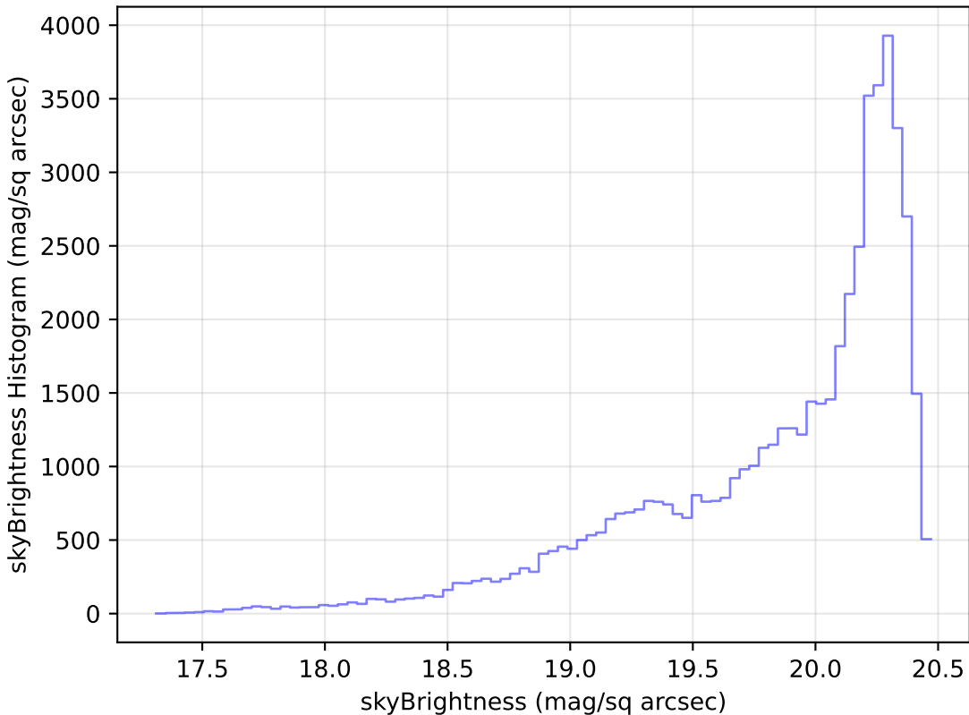
too_100_4v3.4_10yrs Yr 1 i band: skyBrightness Histogram
