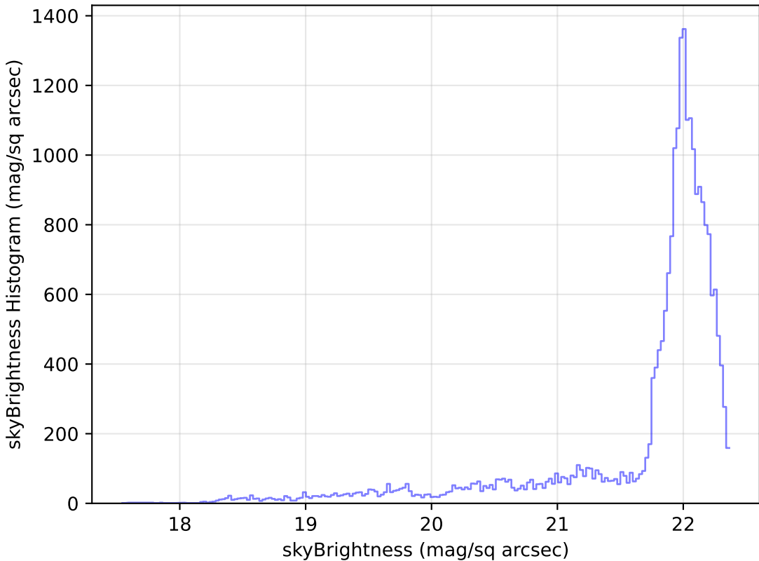
too_100_4v3.4_10yrs Yr 1 g band: skyBrightness Histogram
