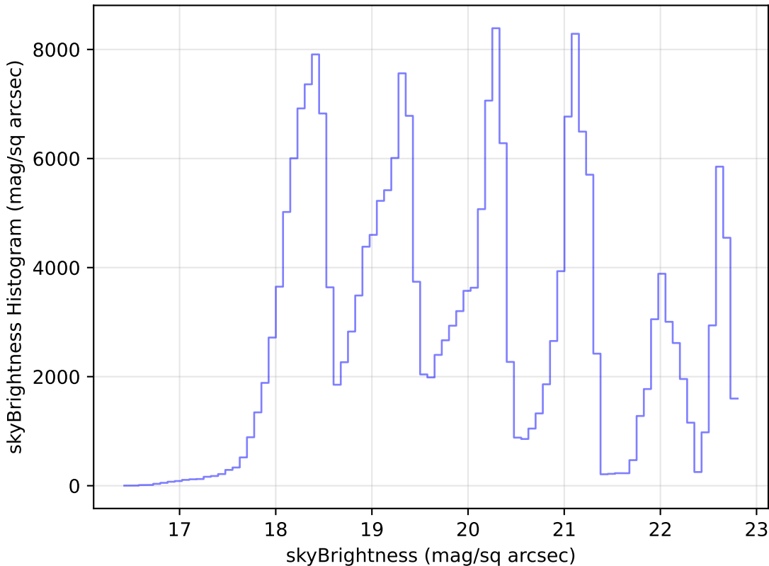
too_100_4v3.4_10yrs Yr 1 all bands: skyBrightness Histogram
